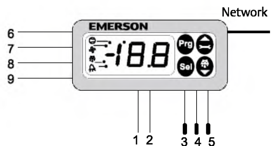
EC2-11x Universal I/O Controller
