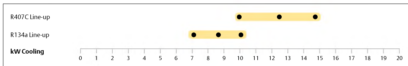
Horizontal Scroll Compressors
