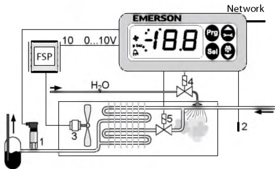
EC2-74x Condenser Controller with fan speed control
