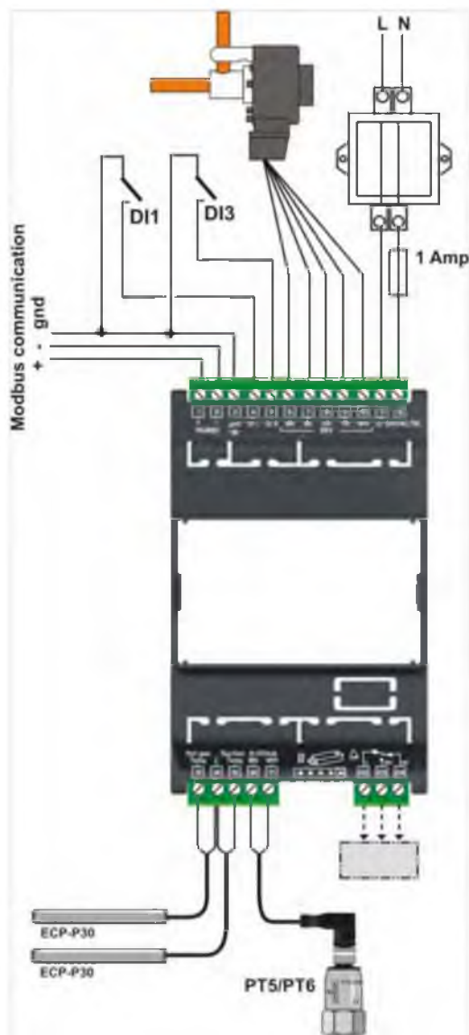
Wiring Diagram EXD-HP1 and EXD-HP2 (Base board)
