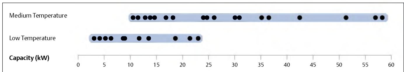
Standard Semi-Hermetic Condensing Units
