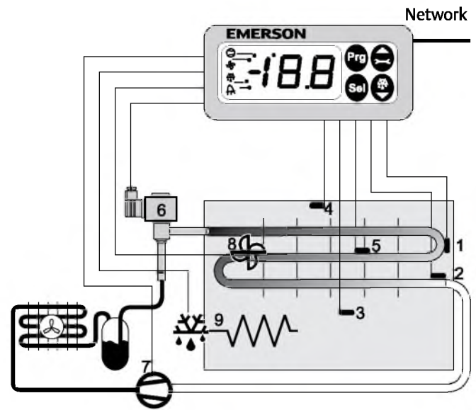
EC2-31x / -39x Case Controller (EX2, Temp/Temp)
